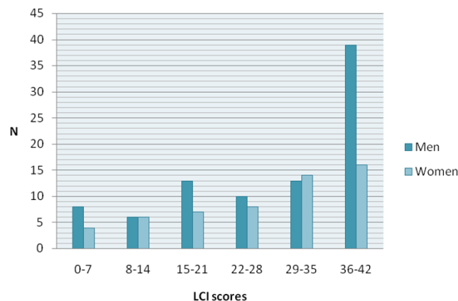
Figure 2 Distribution of the LCI scores (N = 144).
